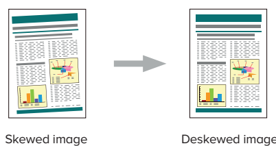
Skewed image
